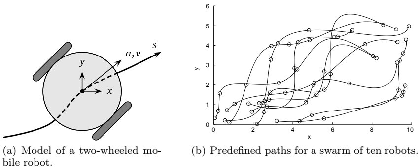
Fig. 3 Model of a two-wheeled mobile robot, and predefined paths for a swarm of ten robots on the cartesian plane. Nodes delimit piecewise cubic spline segments. Initial positions are found in the lower left corner, and final ones in the upper right corner.
