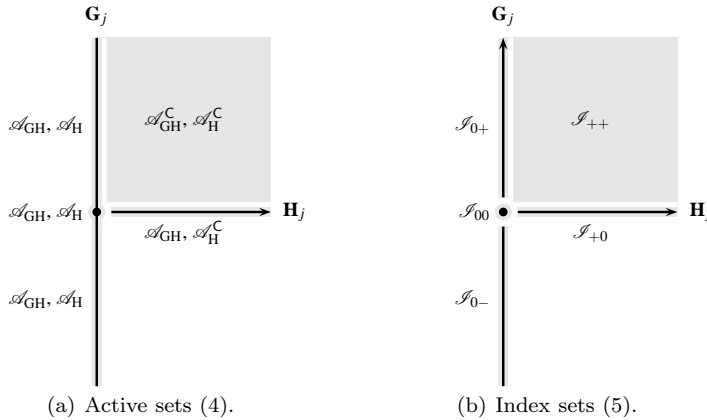
Fig. 1 Active set and index sets in a neighborhood of a feasible point \bar{x} \in \mathbb{R}^n of problem (3).
