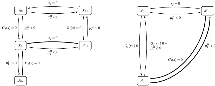
(a) Schematic of the active set algorithm. Emphasized moves may violate MPVC strong stationarity (but not KKT conditions for the subset QP) and trigger a second move as detailed in Section 3.5.
